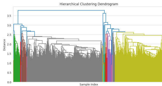
Figure 5: Dendrogram from Hierarchical Clustering
