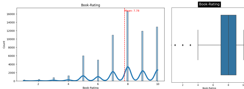
Figure 1: Histogram and Box Plot for the Book-Rating attribute
