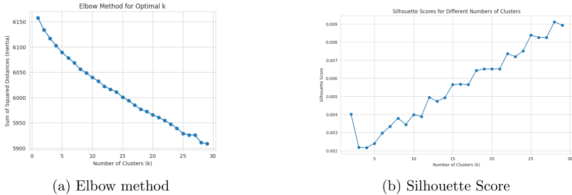
Figure 6: Finding optimal number of clusters
