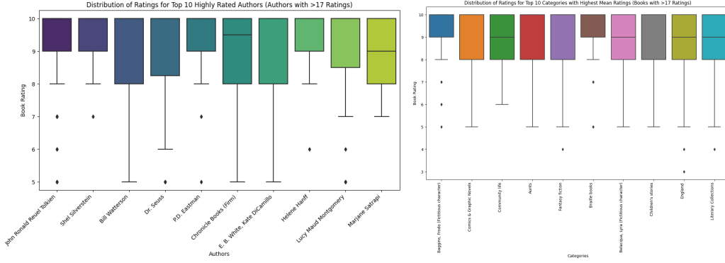
Figure 3: Distribution of Ratings for Top 10 Authors and Categories with Highest Mean Ratings
