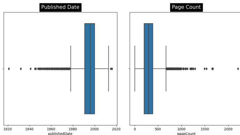
Figure 2: Box Plot for 'publishedDate' and 'pageCount'
